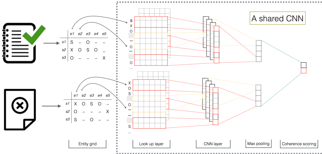
Figure 2: Neural model for coherence scoring and the pairwise training method [taken from our previous work [14]].
